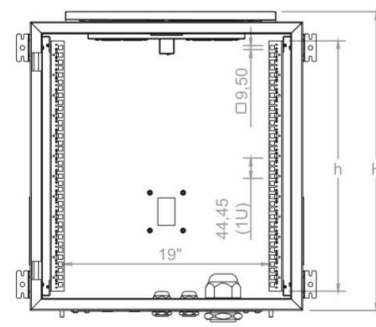
Inside view
