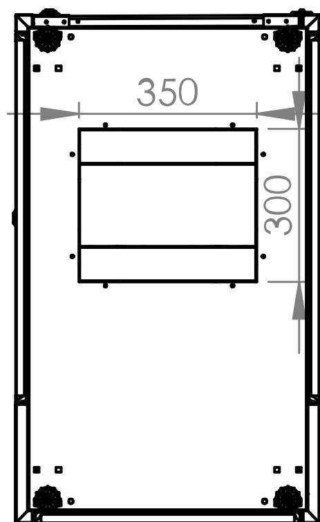
Bottom view
