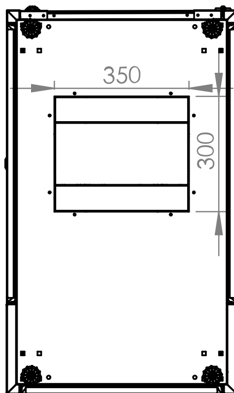
Bottom view
