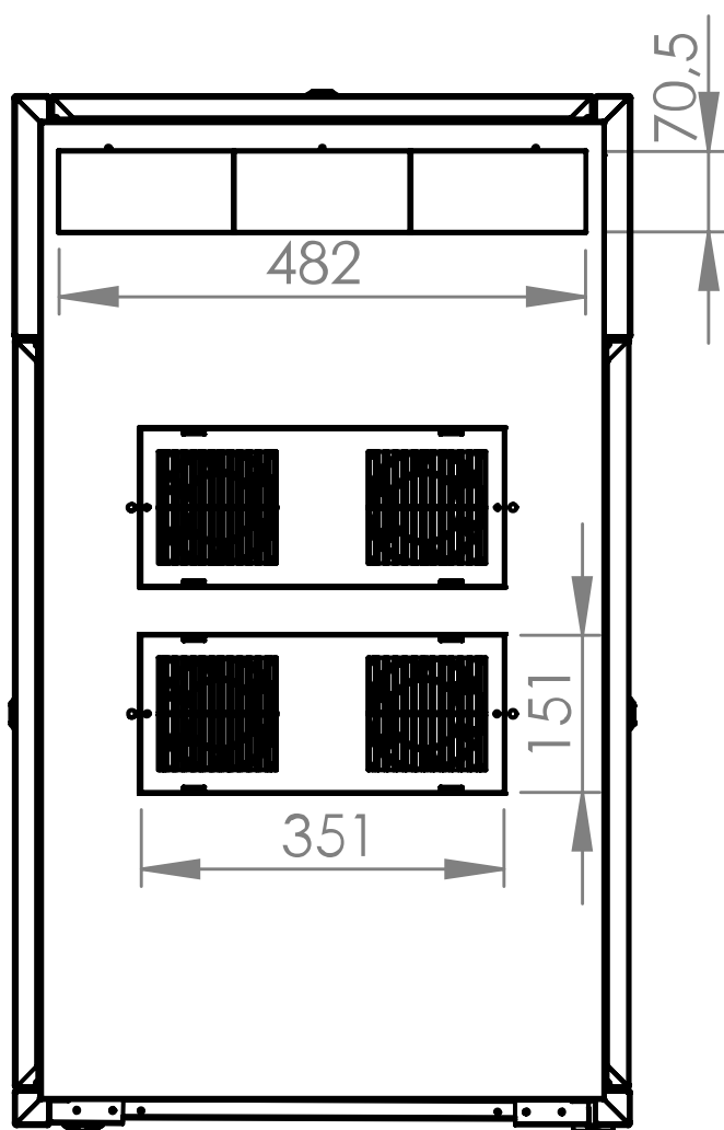
Top view
