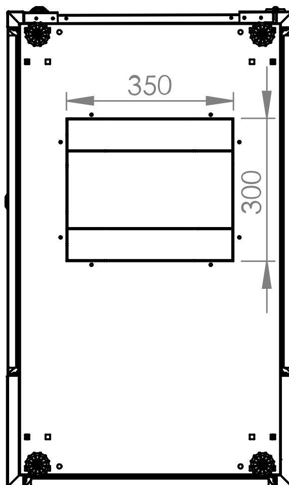
Bottom view
