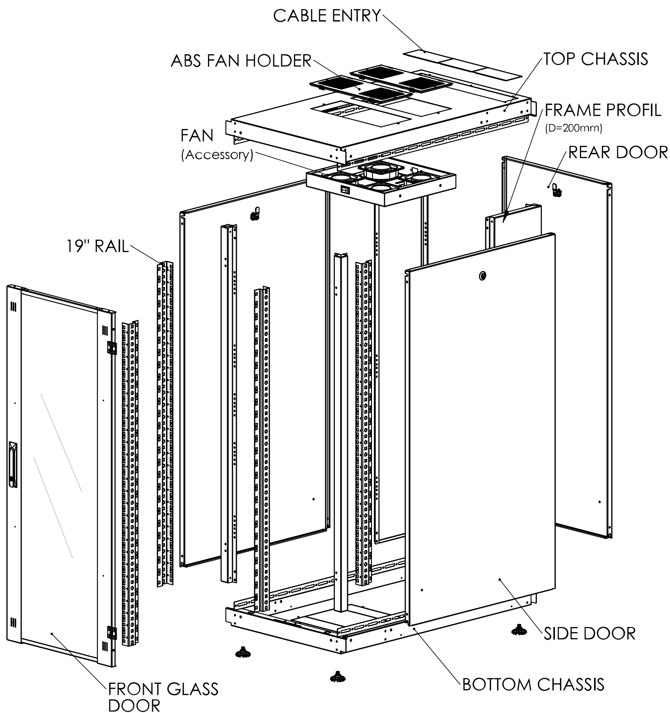
Exploded view
