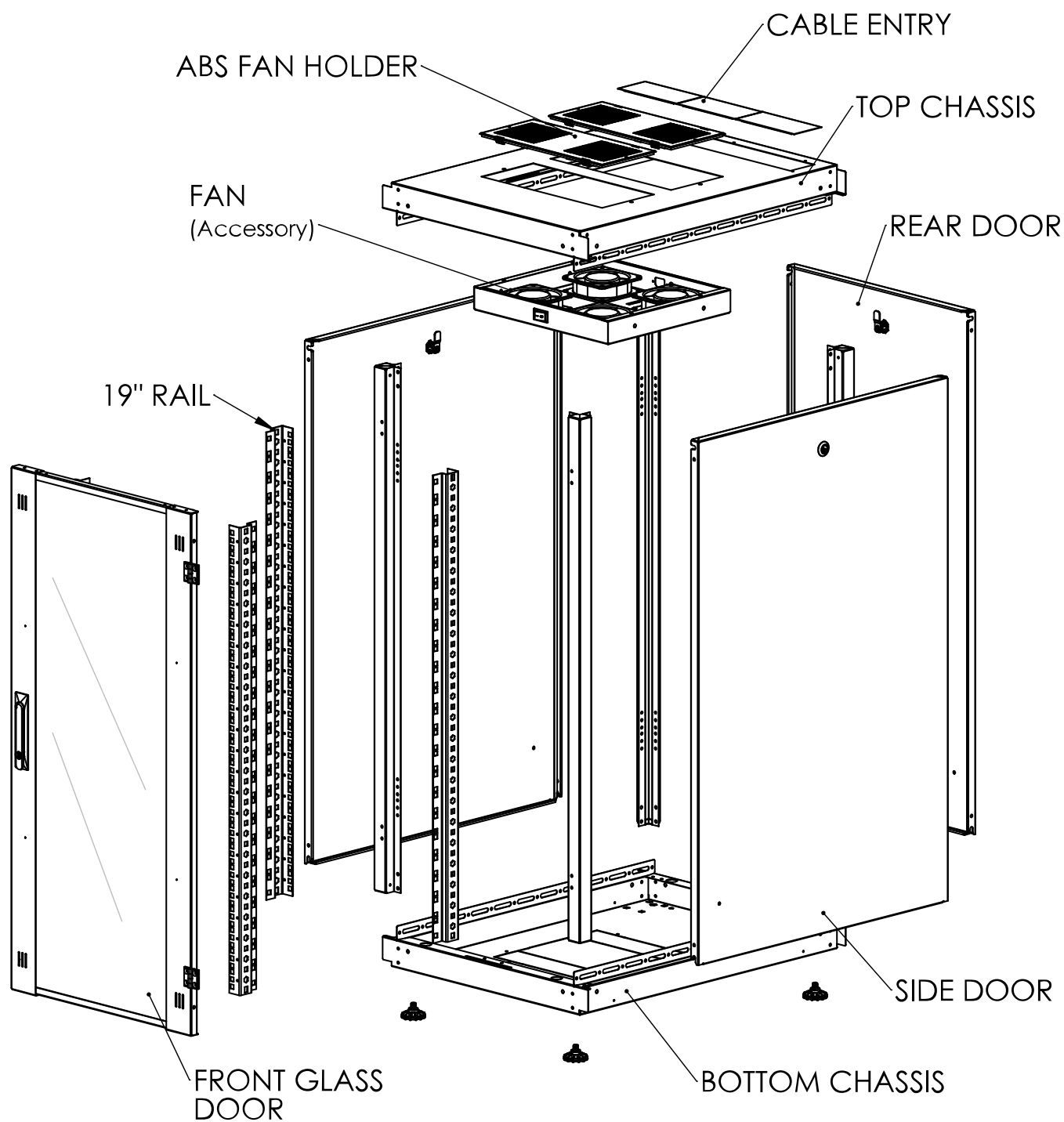
Exploded view
