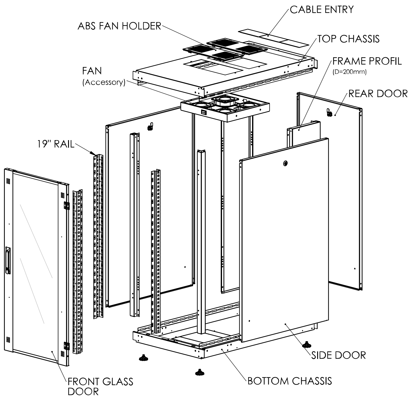
Exploded view
